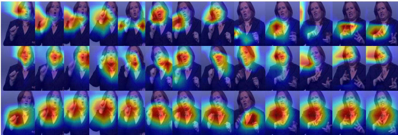
Fig. 10. Saliency maps showing the CNN-LSTMs highest activations. Generated with Grad-Cam [76], from top to bottom: sign-gloss stream, mouth shape stream, hand shape stream. It can be seen that the hand model focuses on the right hand, the mouth model on the mouth and the sign-gloss swaps between both hands and the mouth.
