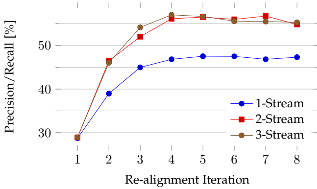
Fig. 8. mouthings (precision/recall), clean conditions: compare 1stream against 2stream (gloss and mouth) and 3stream (gloss, mouth, hand)
